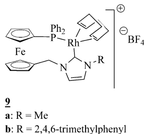
Figure 5. Previously described Rh I complexes with an imidazol-2-ylidene moiety. [4]
