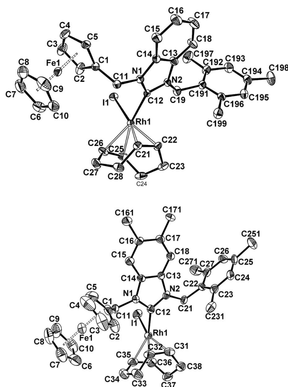
Figure 4. ORTEP views of 8a (top) and 8b (bottom). Ellipsoids are shown at the 50% ( 8a ) or 30% ( 8b ) probability level. All hydrogen atoms are omitted for clarity.
