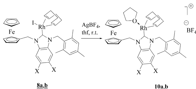
Scheme 5. Generation of cationic \text{Rh}^{\text{I}} complexes bearing monodentate NHC ligands.
